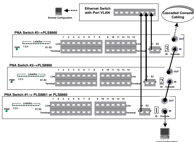
Figure 4 Cabling of more DYNAMIX DH - 114/DYNAMIX DH - 114 M by Ethernet Switch
